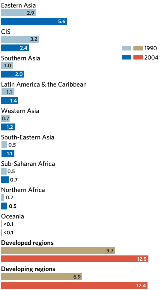
Emissions of carbon dioxide (CO 2 ), 1990-2004 (Billions of metric tons)
