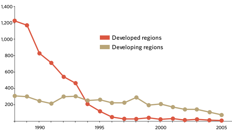
Consumption of all ozone depleting substances, 1989-2005 (Thousands of metric tons of ozone-depleting potential)
